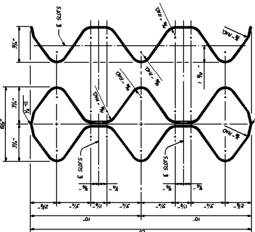
SECTION THRU TUBULAR BEAM GUARDRAIL SECTION THRU CORRUGATED BEAM GUARDRAIL
